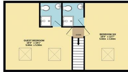
ORIGINAL DESIGN (2ND FLOOR)
